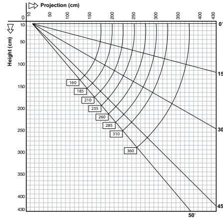
Australia R-90 Cross Over Arms
