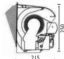
Global 2020 with Hood Wall/Face Fix
