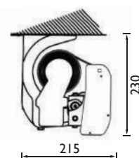
Global 2020 Semi-Cassette with No Hood Ceiling/Top Fix
