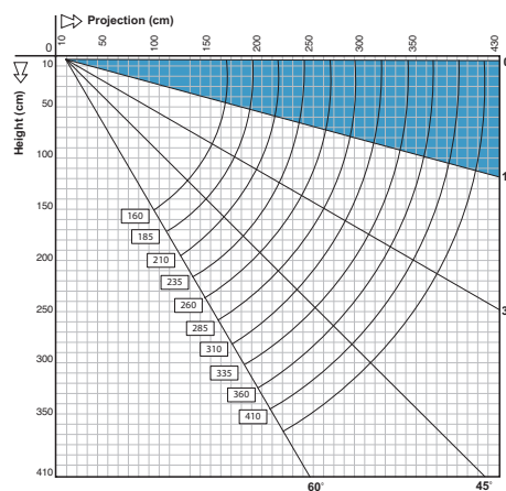
Global 2020 with Hood Wall/Face Fix
